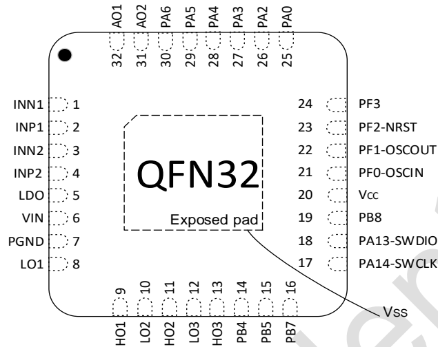
图 3-1 QFN32 Pinout1 PY32MD310K1xU (Top View)
